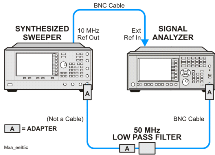
Figure 4-1. Second Harmonic Distortion Test Setup
